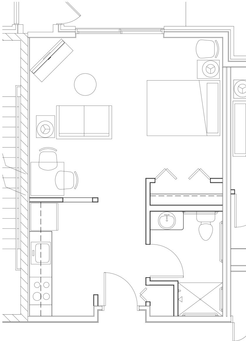
5 ASSISTED LIVING- STUDIO (UNIT K) A2.1 1/4" = 1'-0"
