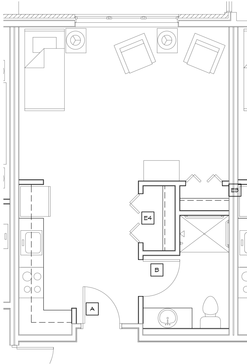
3 MEMORY CARE - STUDIO (UNIT D) A2.1 1/4" = 1'-0"
