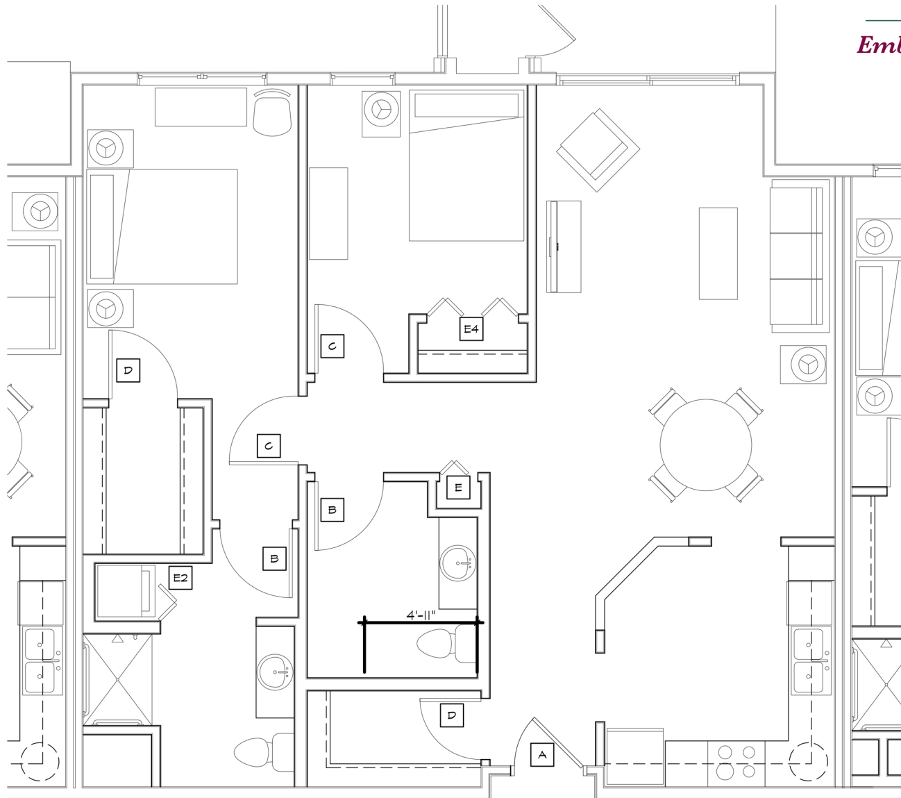
2 INDEPENDENT LIVING-TWOE BEDROOM (UNIT 1) A2.4 1/4" = 1'-0"
