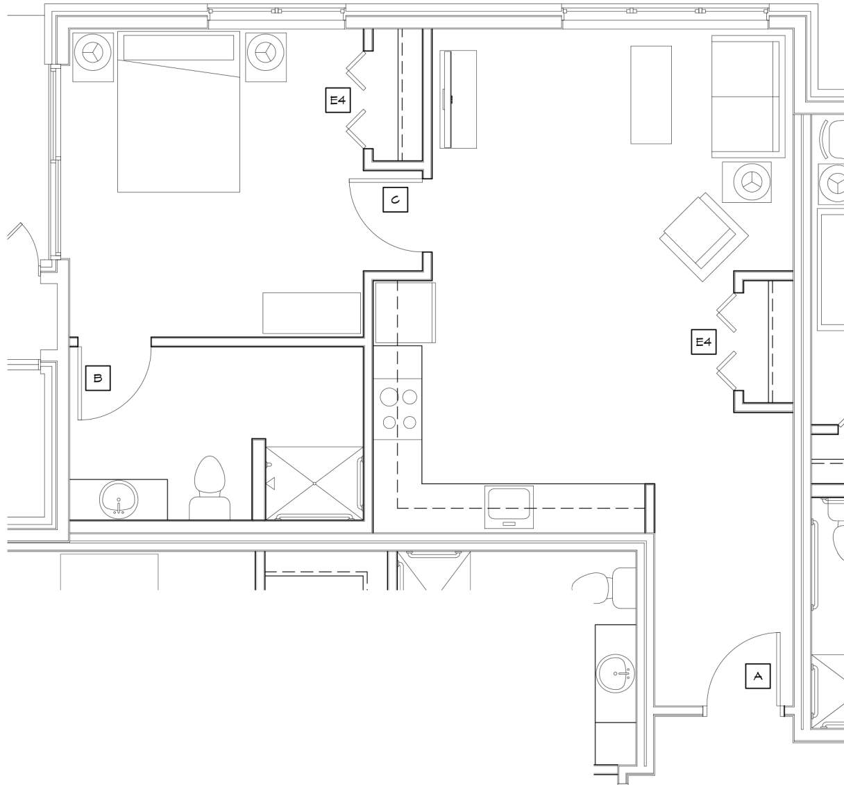
2 ASSISTED LIVING- ONE BEDROOM (UNIT P1) A2.2 1/4" = 1'-0"
