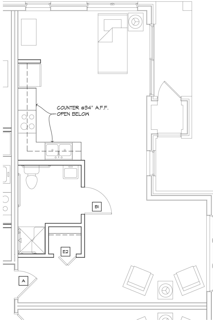
10 A2.0 ASSISTED LIVING HC- STUDIO (UNIT N) 1/4" = 1'-0"
