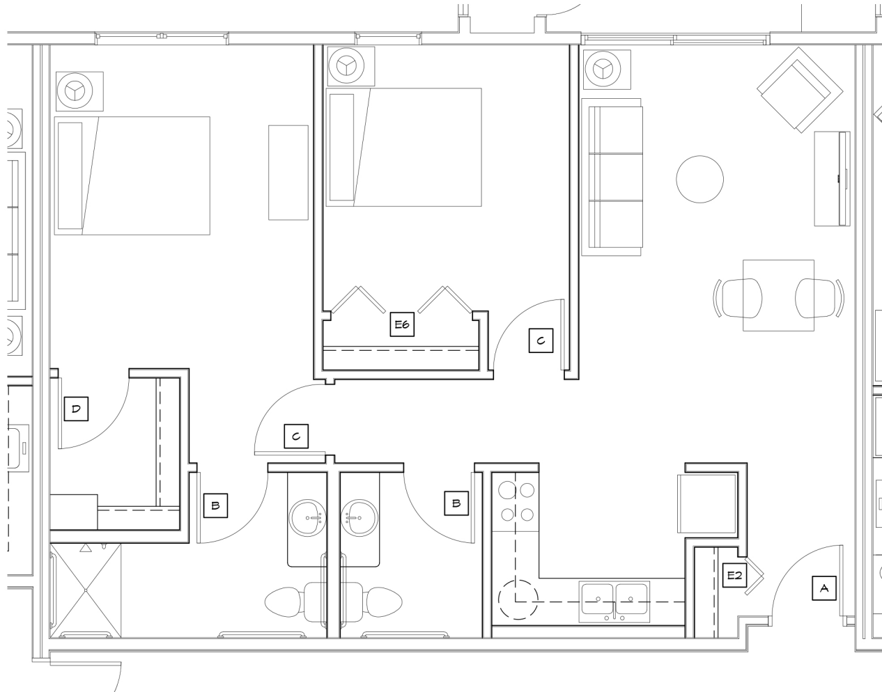
4 A2.3 ASSISTED LIVING- TWO BEDROOM (UNIT LI) 1/4" = 1'-0"
